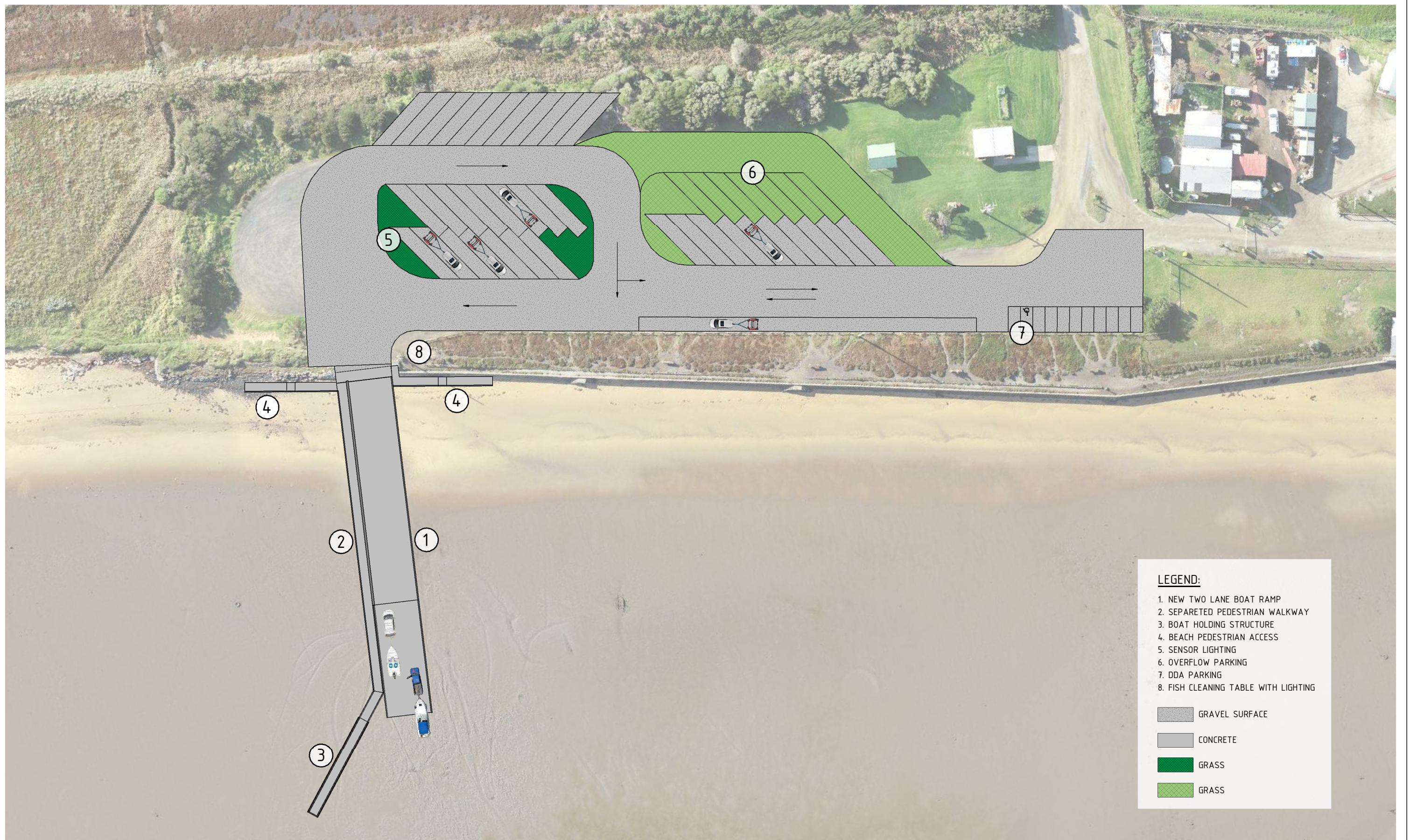
1 FULL PLAN - STR + CIV 1 : 750
