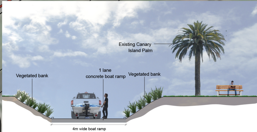
Section A: Boat launch ramp (Not to scale)
